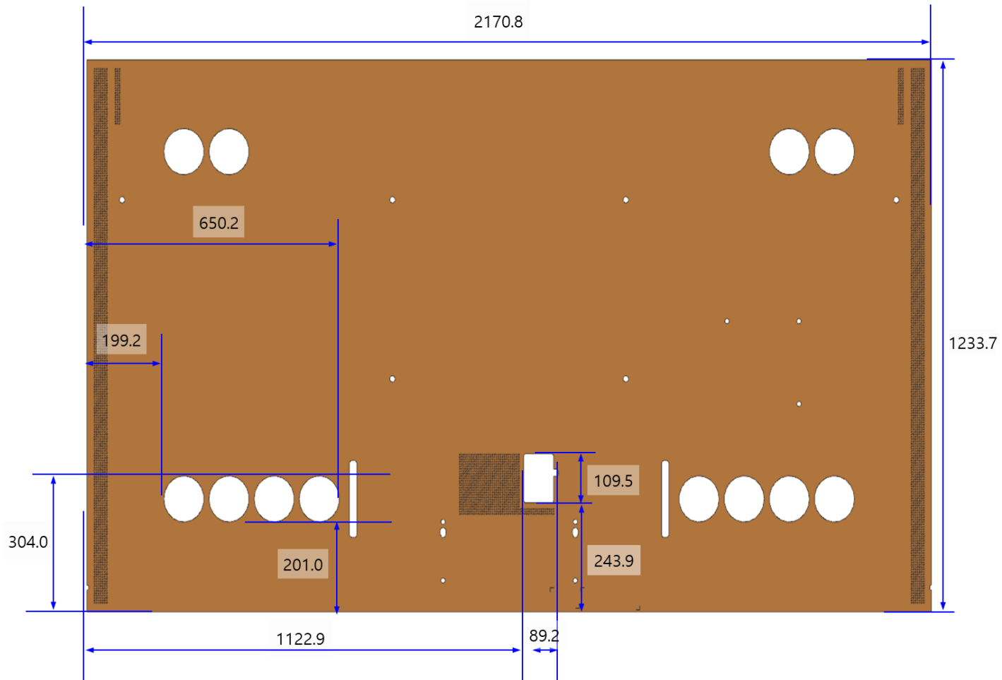
QN100B 98" Cover and Rear-View Dimension
