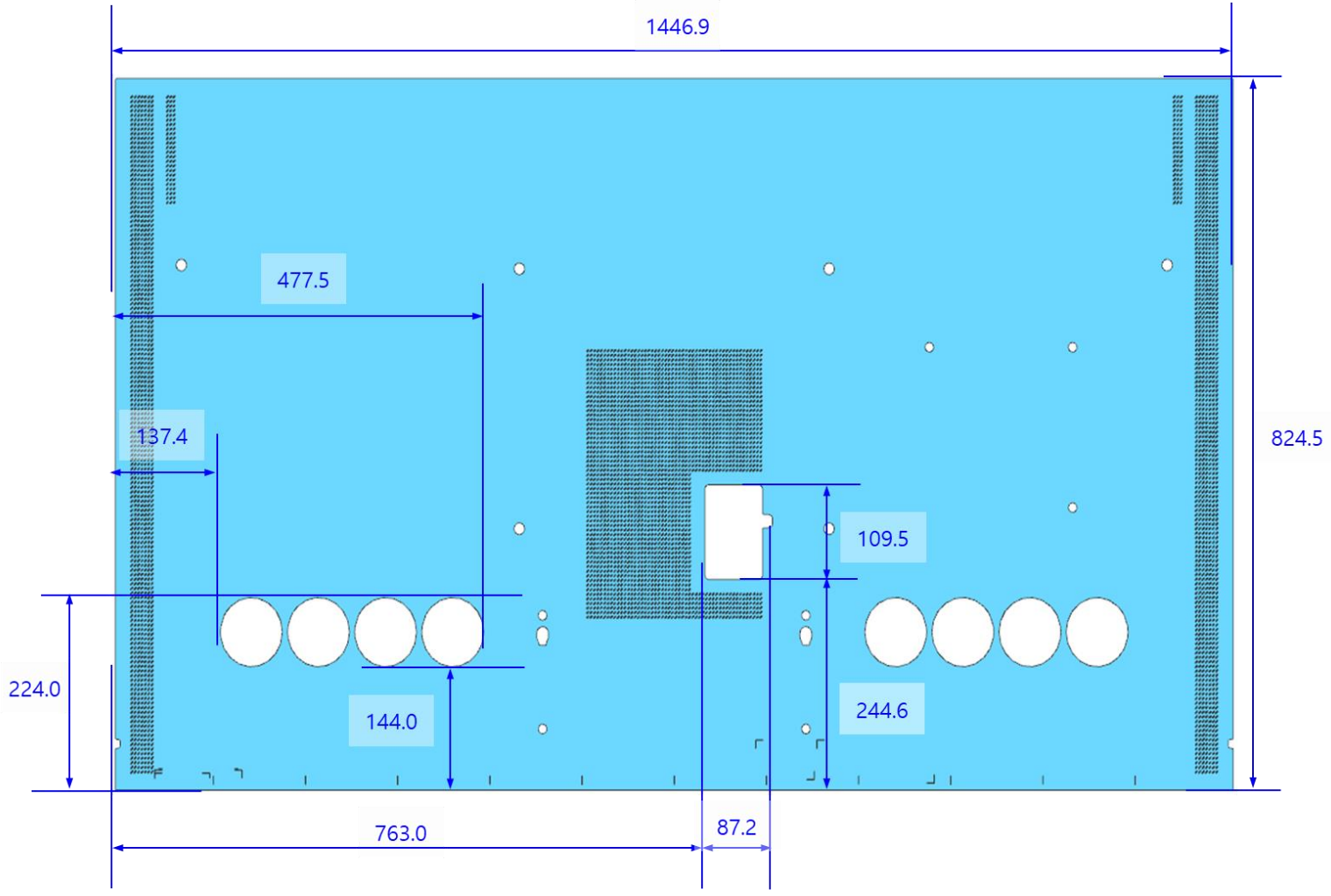
QN95B 65" Cover and Rear View Dimensions
