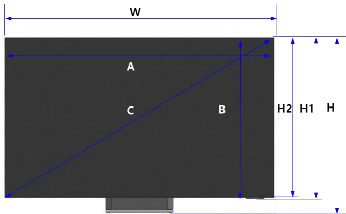
SET Front View *Include Rubber-foot
