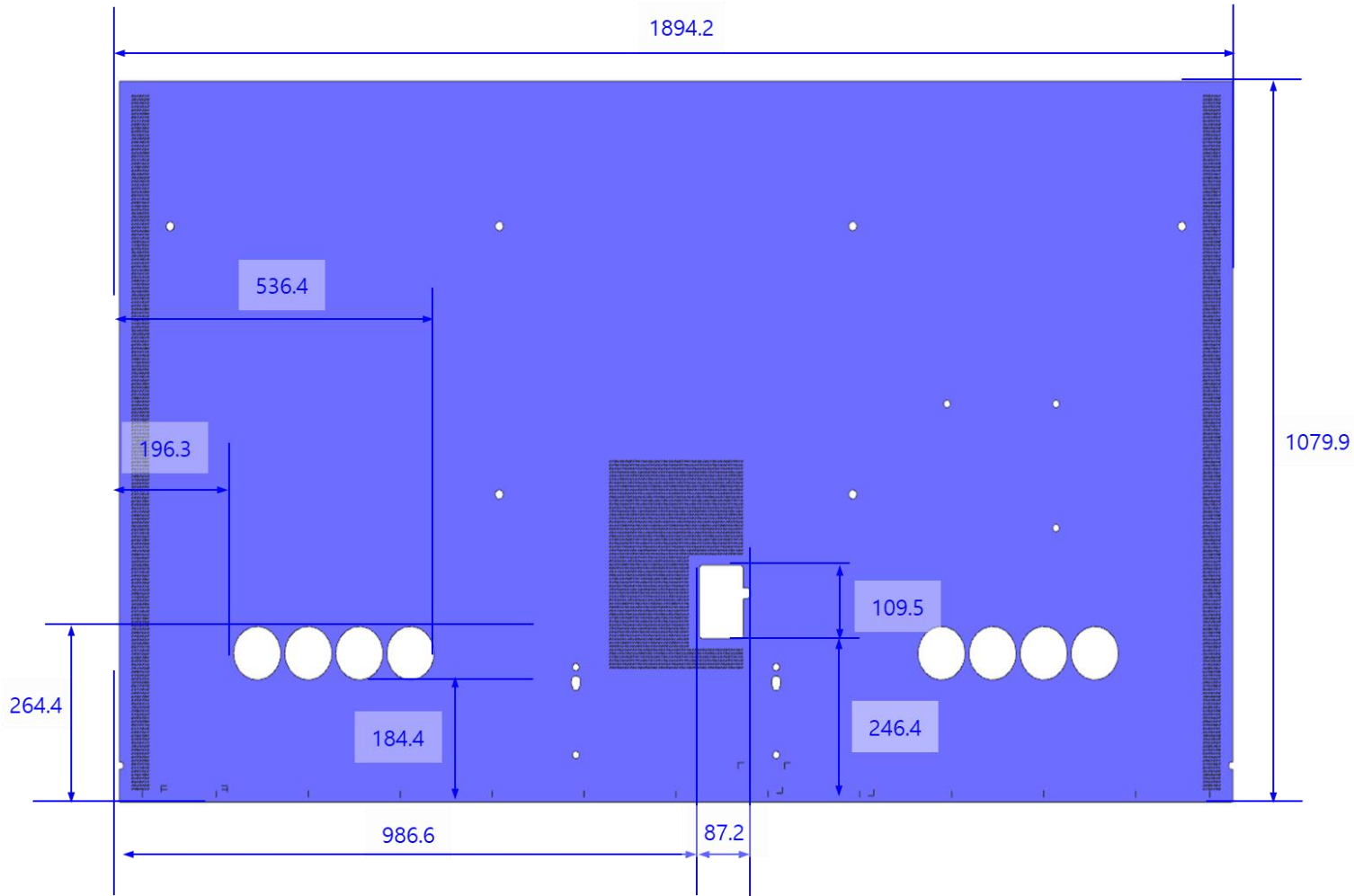
QN95B 85" Cover and Rear View Dimensions
