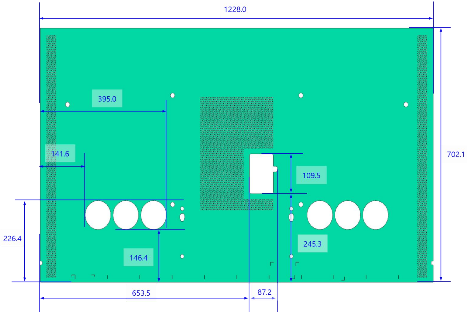
QN95B 55" Cover and Rear View Dimensions
