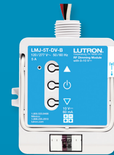
LMJ-5T-DV-B (0–10 V dimming)
