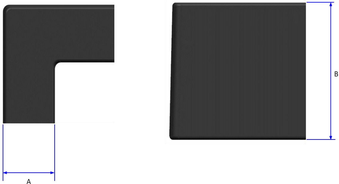
LS03FA Bezel Dimensions
